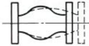
2. Axial Elongation
