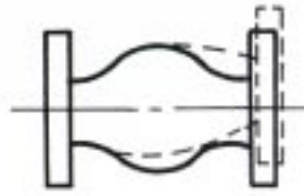
3. Transverse Movement
