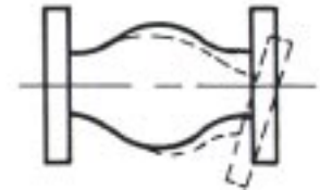
4. Angular Deflection
